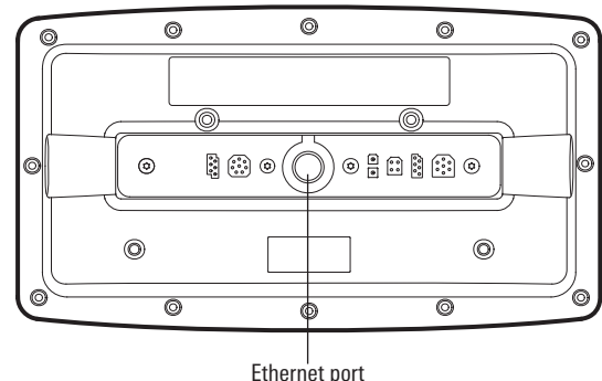
800 Series/900 Series with Round Ethernet Port
