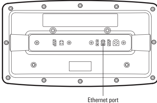
Cable Collector with Ethernet
