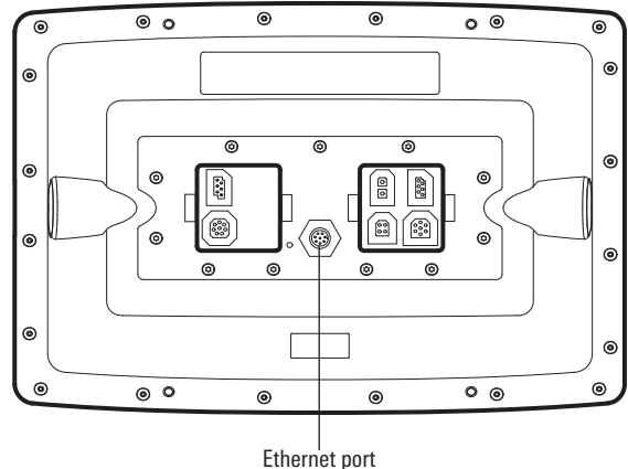
800 Series/900 Series with Round Ethernet Port
