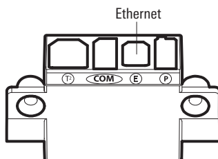
Cable Collector with Ethernet
